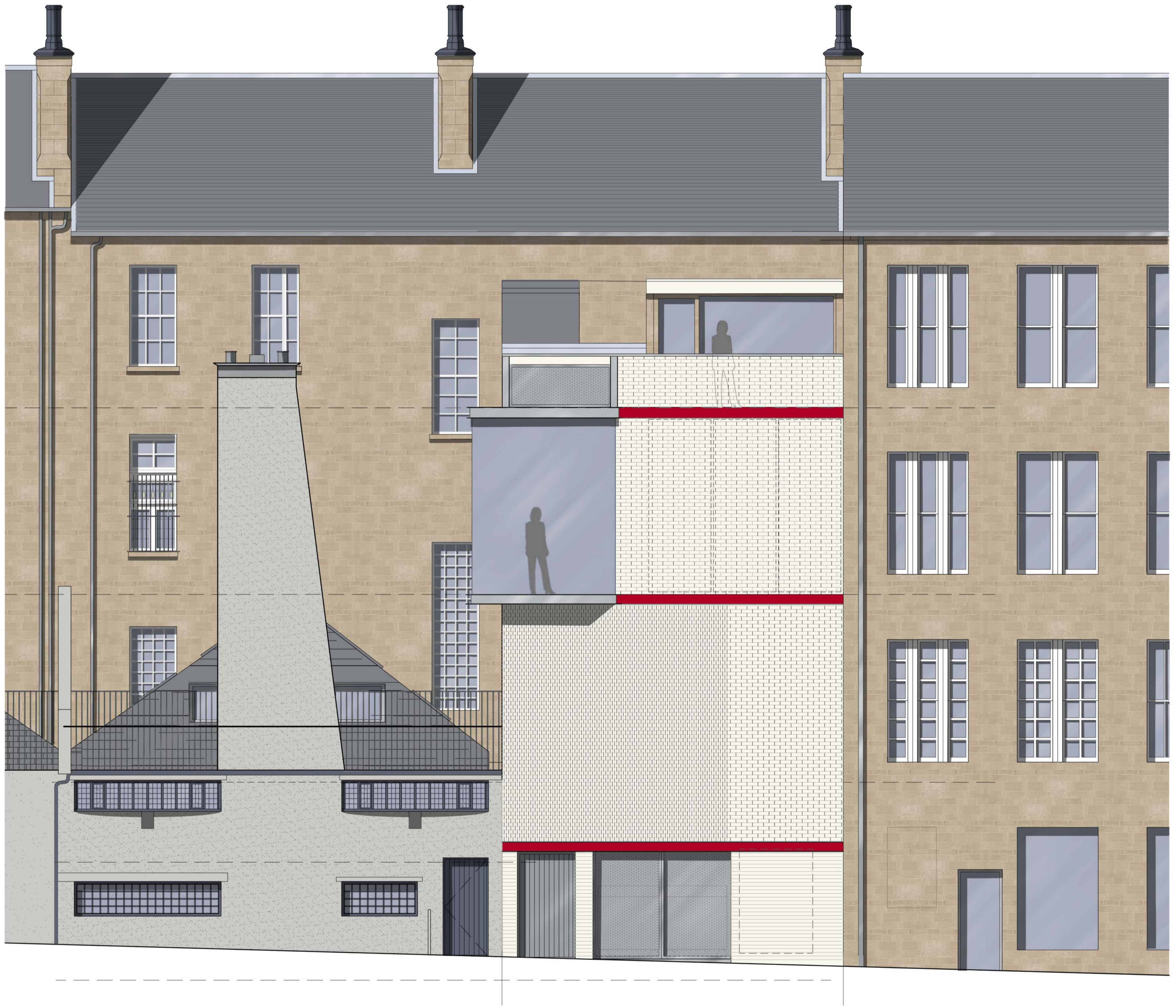
SOUTH ELEVATION
